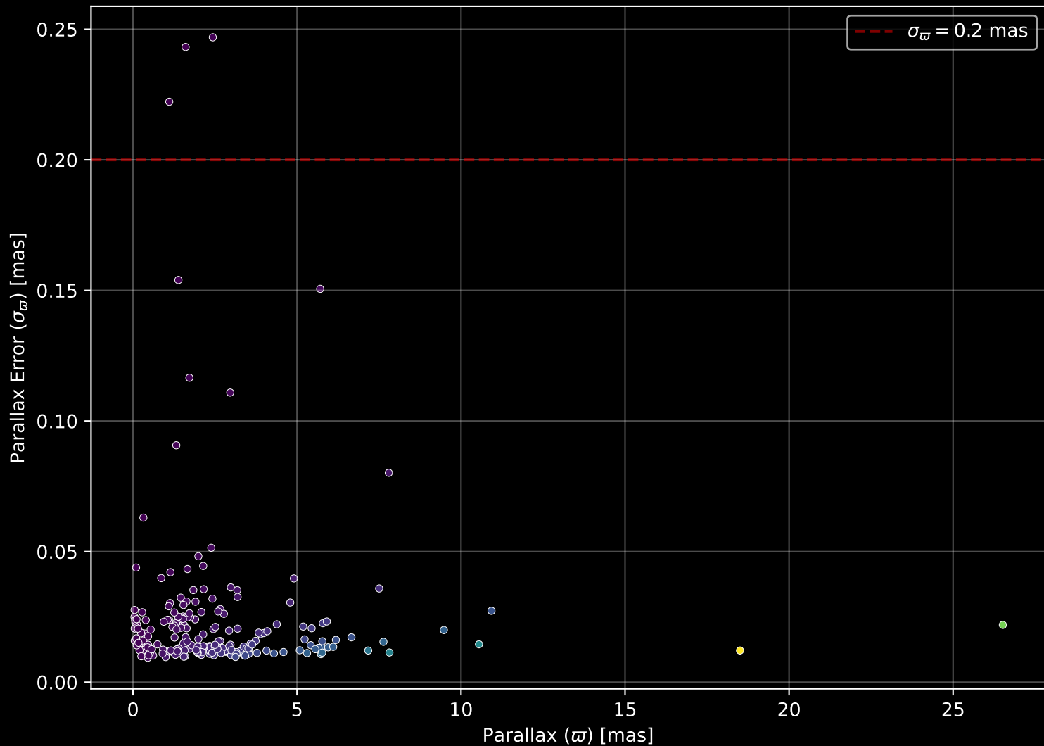
APOGEE DR17 Field: [071+62_btx] Parallax Quality (n= 210)
