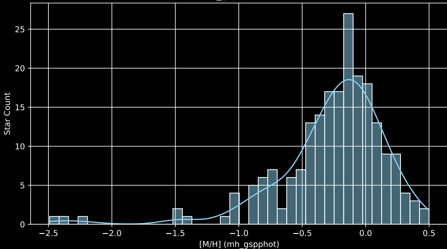
APOGEE DR17 Field: [071+62_btx [M/H] (mh_gspphot) (n= 209)
