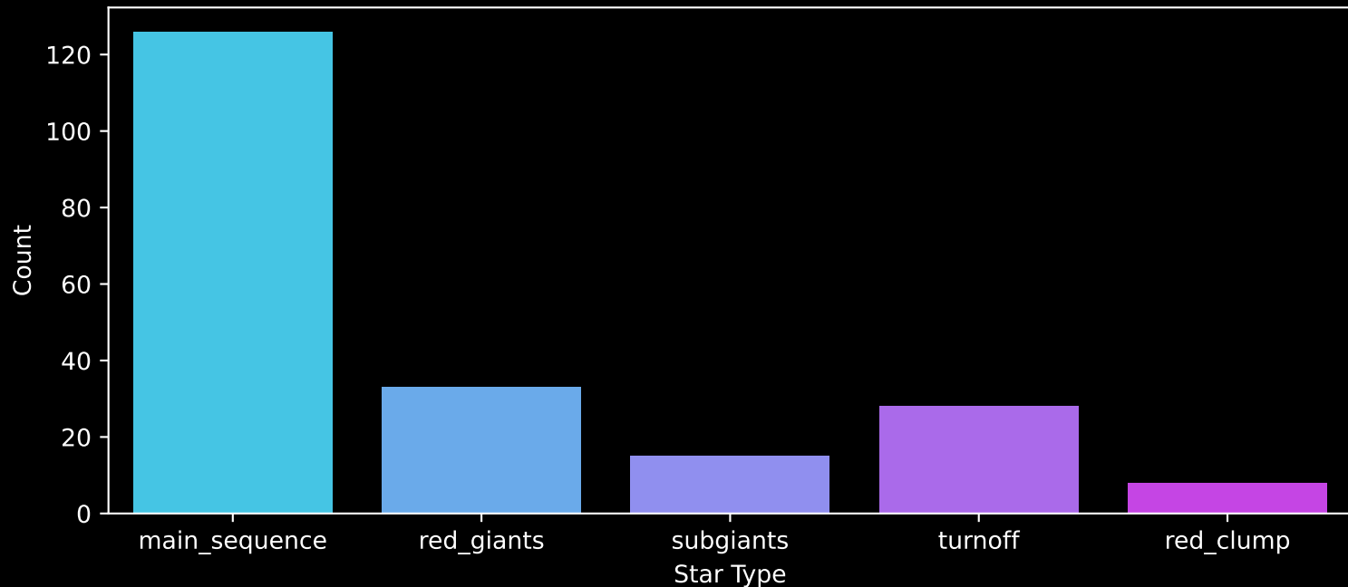
APOGEE DR17 Field: [071+62_btx] Count plot of Star Type
