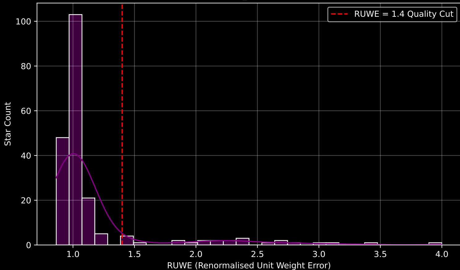
GAPOGEE DR17 Field [071+62_btx] RUWE Distribution (n= 202)
