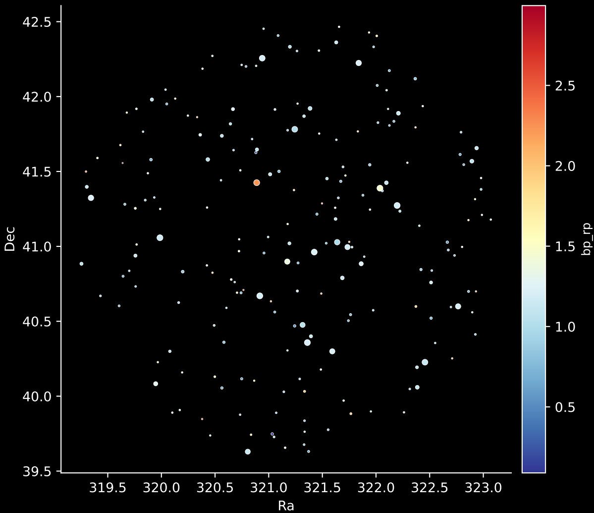
APOGEE DR17 Field: [071+62_btx] Stars: 210
