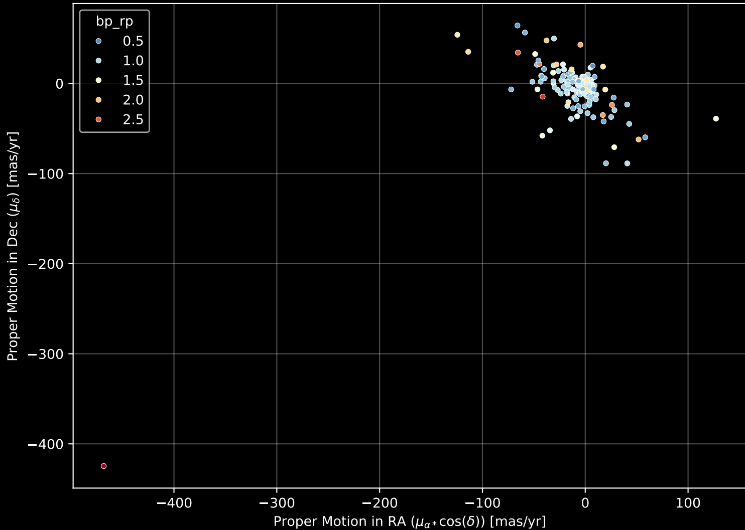
APOGEE DR17 Field: [071+62_btx] Proper Motion Diagram (n= 210)
