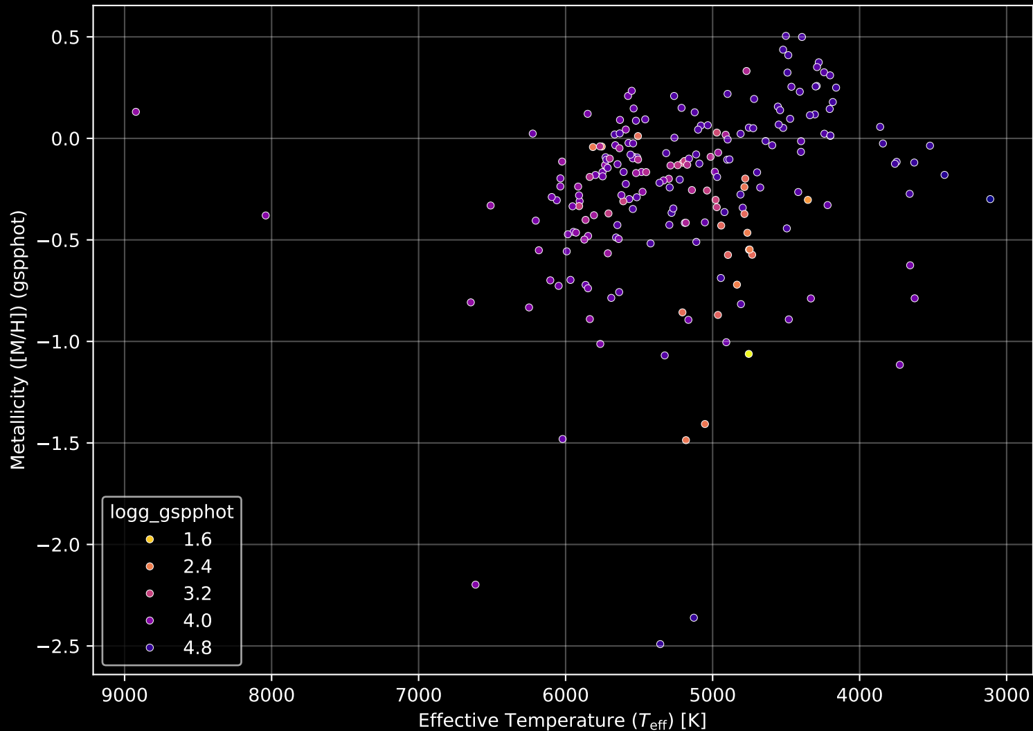
APOGEE DR17 Field: [071+62_btx] Stellar Population Parameters (n= 210)
